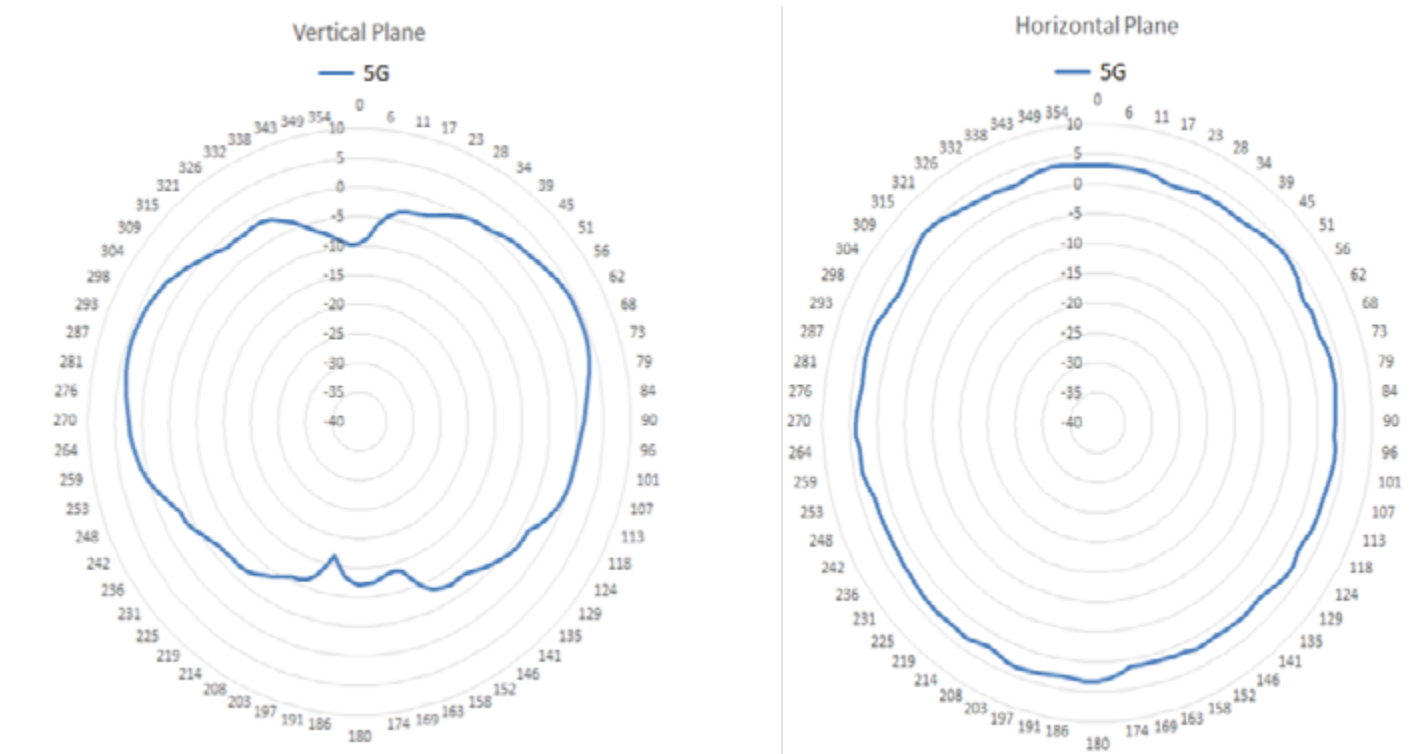
AP505i Antenna Radiation Patterns – 5.0GHz
